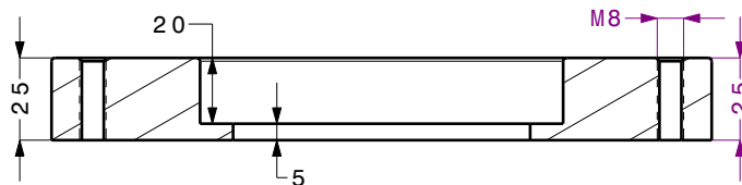
Section view V-V Scale: 2:5
